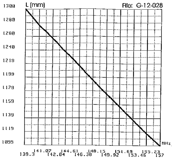
TYPICAL TUNING DIAGRAM vs FREQUENCY
