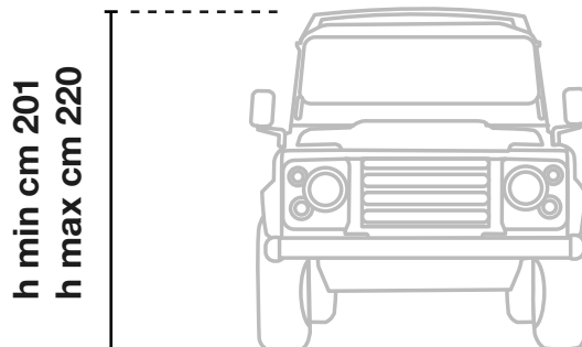
Changing room for 4x4 High-Wagon
