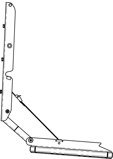
OPEN POSITION
