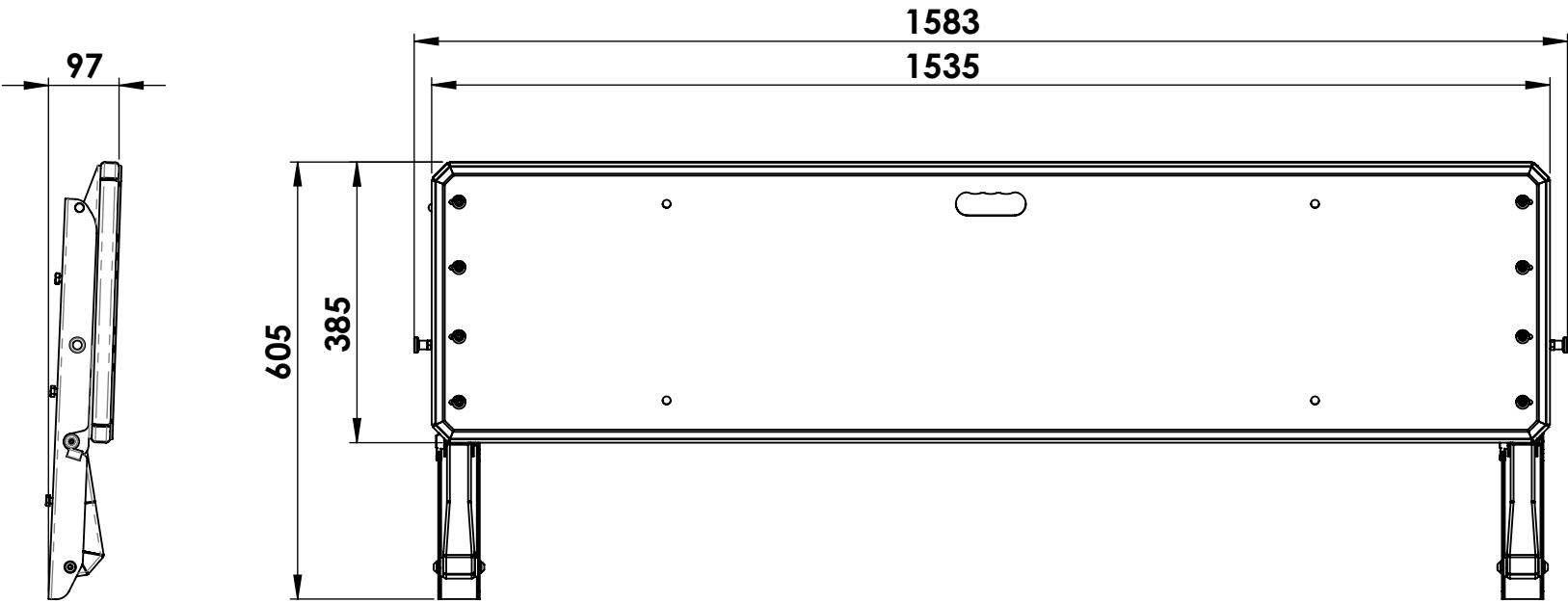
CLOSED POSITION
