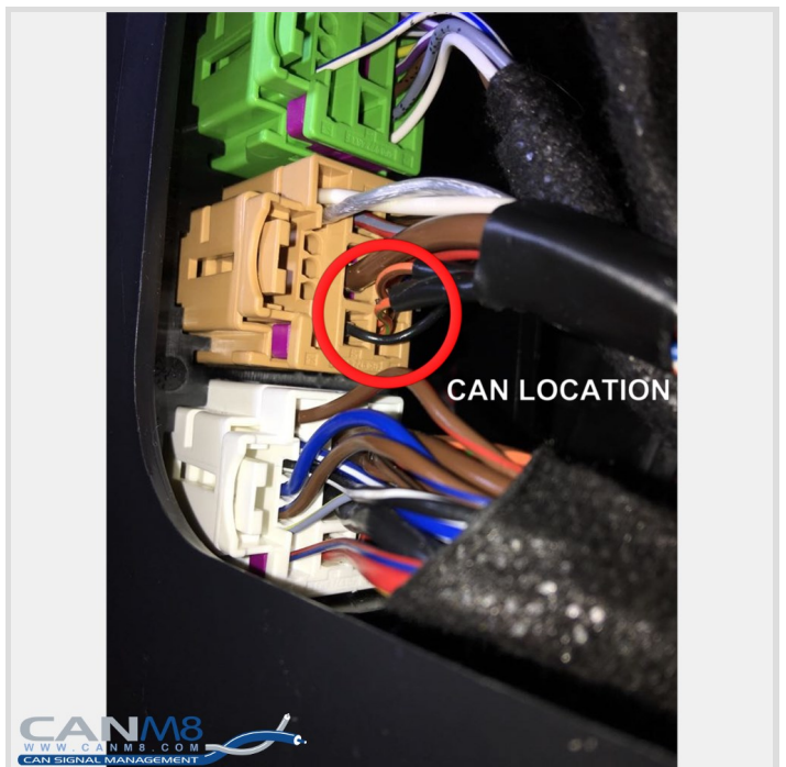
CAN wiring
